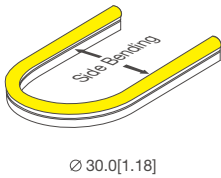
Bending Diameter
