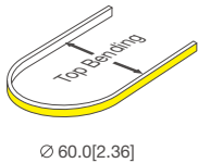
Bending Diameter
