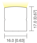
Sectional view
